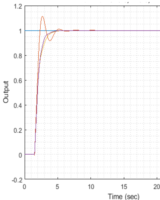
Fig. 4: Waveforms on Giving a Step Input
