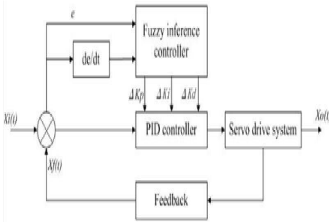
Fig. 1: Adaptive PID Control System Design Structure
