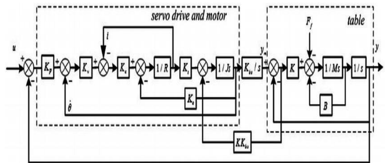
Fig.1: Feed Servo System
