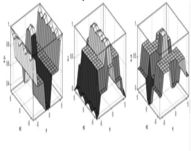
Fig. 2: rule of fuzzy control of the three parameters of K_p , K_i , K_d
